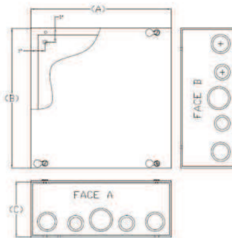
Fig.- Shows the Drawing of S C BOX 664
