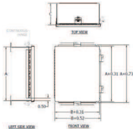
Fig.- Shows the Drawing of MDHC BOX 884
