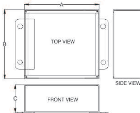
Fig:- Shows the Drawing of W.P. BOX 864
