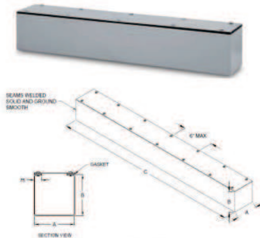
Fig.- Shows the Drawing of WPT 6624
